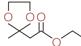
ethyl (2-methyl-1,3-dioxolan-2-yl) acetate
